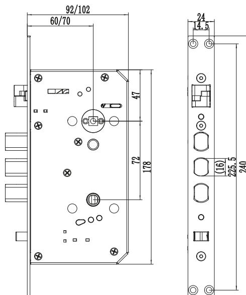
824C Mortise
