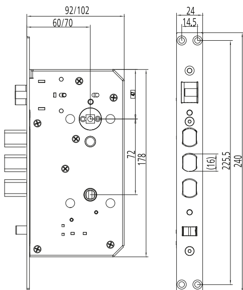
924C Mortise
