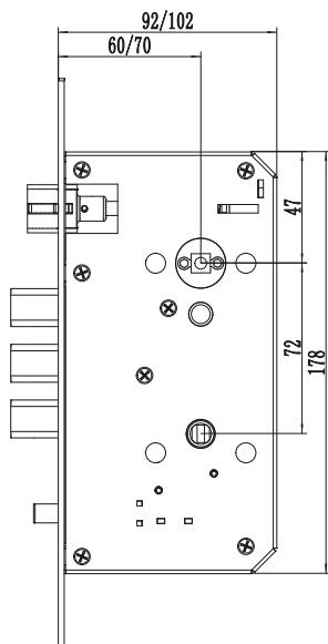
824 Mortise
